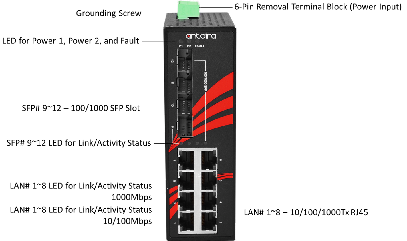
Figure 2.2 - Front View Panel
