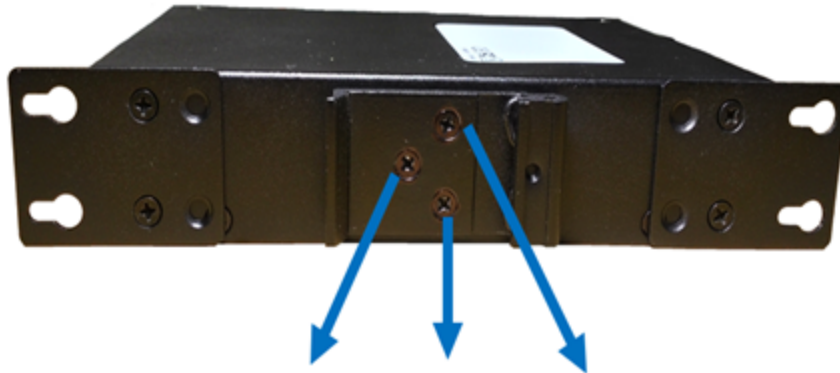
Figure 3.4 - Remove DIN-Rail bracket from the Switch and place the wall mounting brackets
